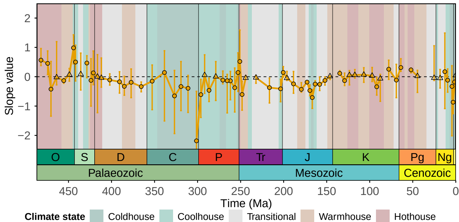
(b) Southern Hemisphere
